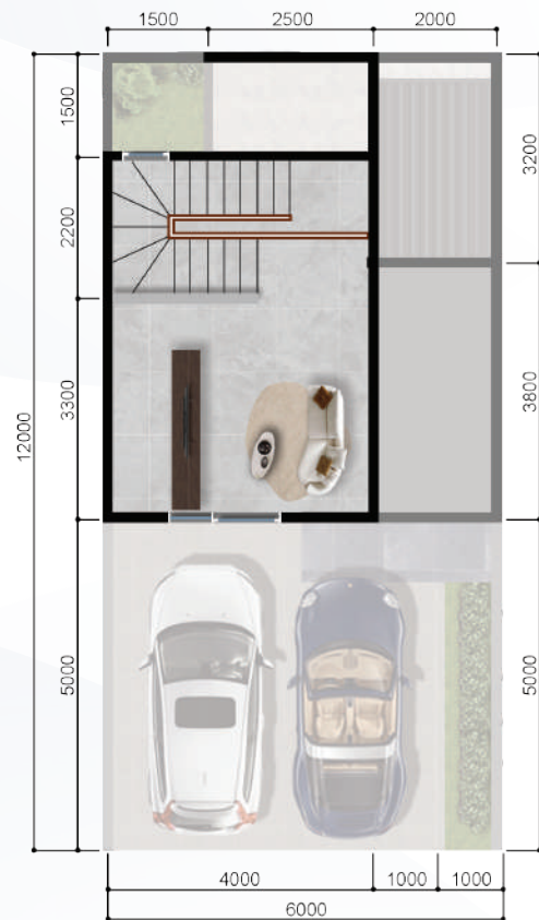
3 rd Floor Plan
